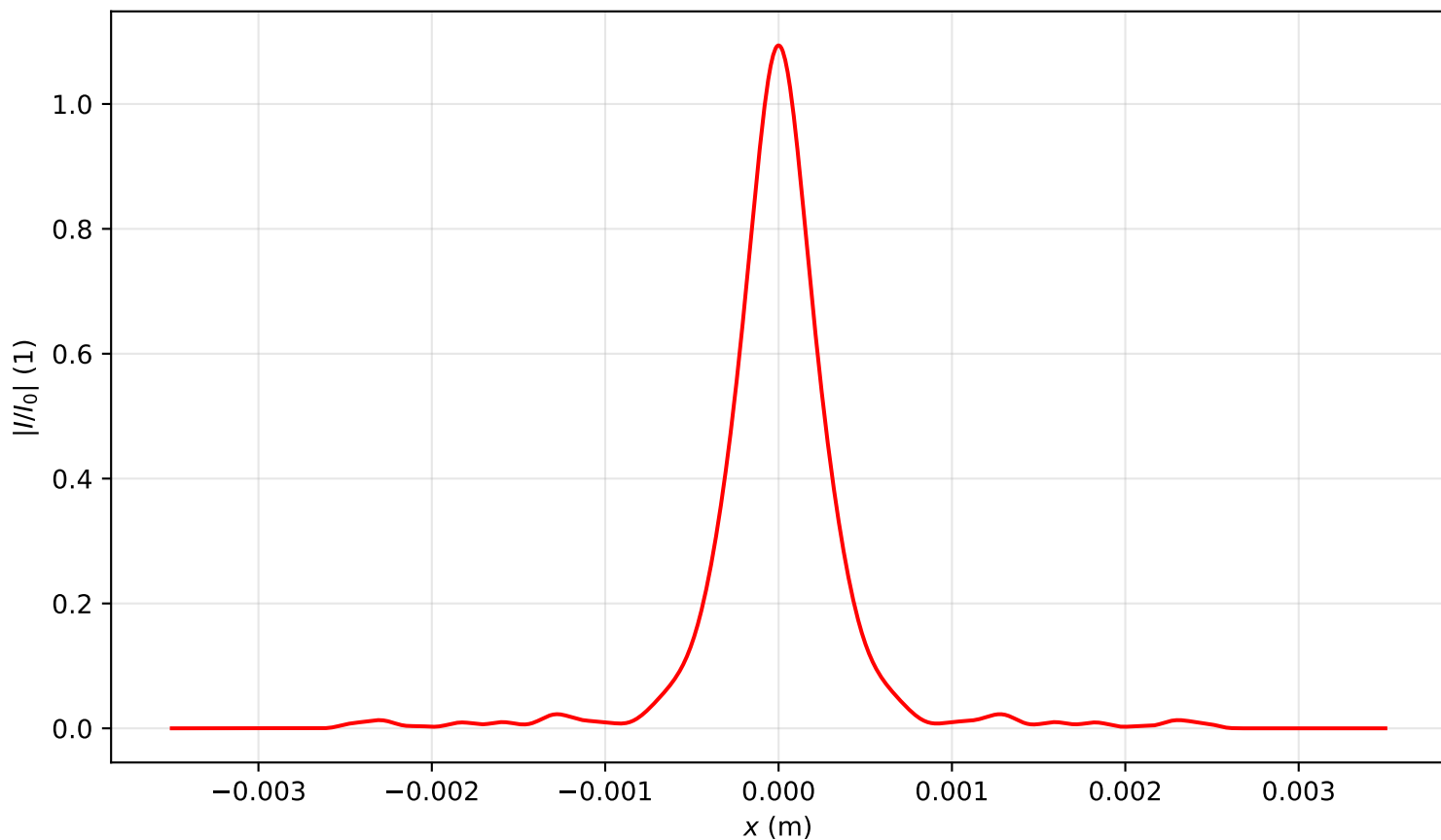
Intensity profile I(x, y = 0, z = 3.821)/I_0 , \text{Pin}=2.0\text{Pcr} , artificial time
